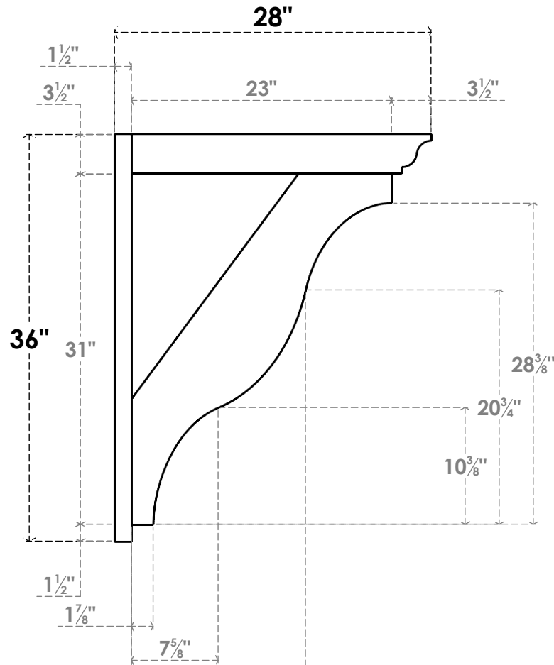
SIDE PROFILE
